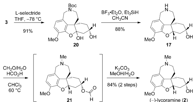
Scheme 7. Synthesis of 2 .
